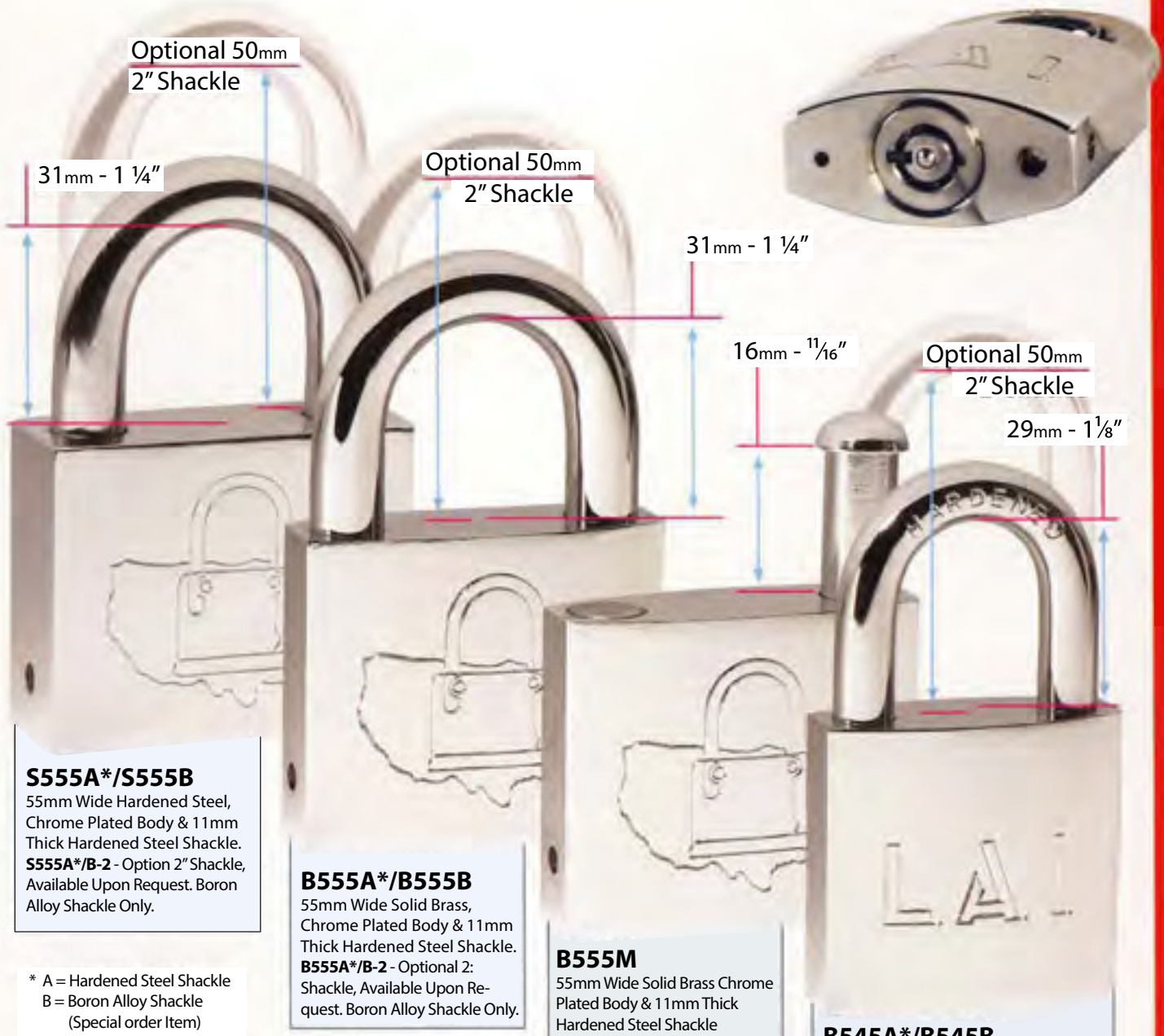
B545A*/B545B 45mm Wide Solid Brass, Chrome Plated Body & 9mm Thick Hardened Steel Shackle. B545*/B-2 - Optional 2" Shackle, Available Upon Request. Boron Alloy Shackle Only.
